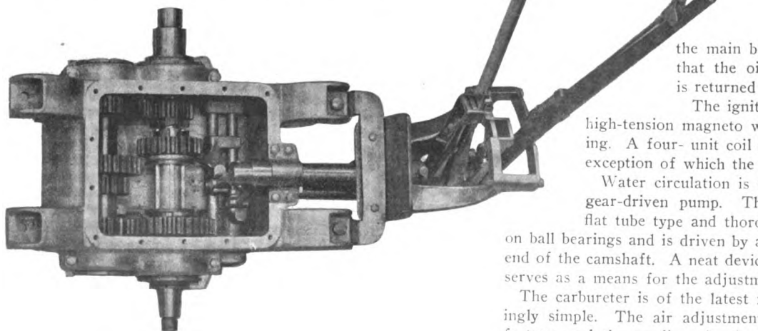
View from Above of Gears and Shifting Levers.
